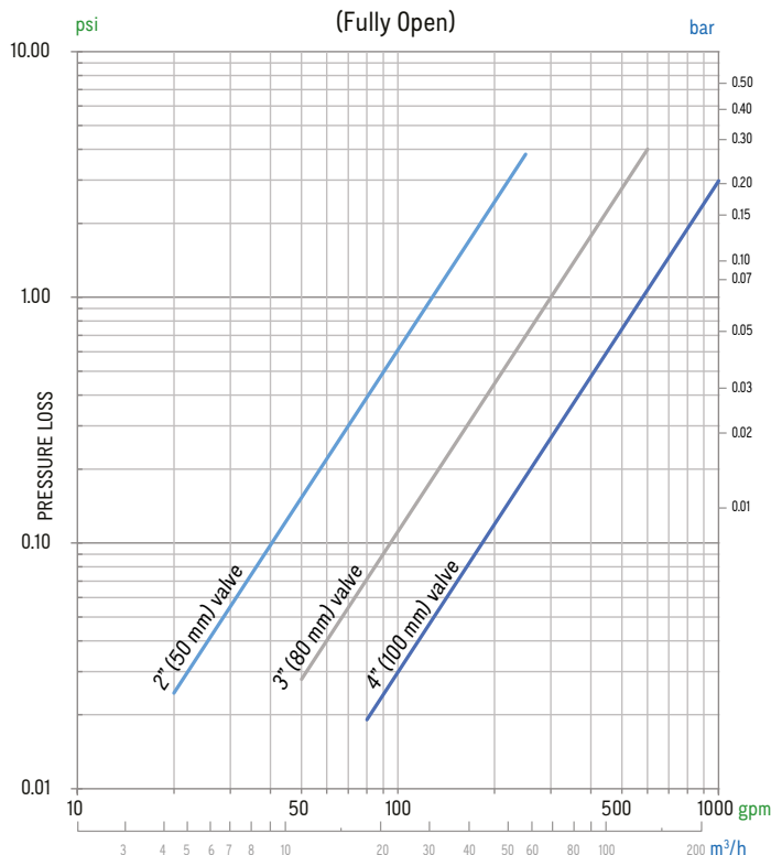
Pressure Loss Data 1000 Series Inline Valves (Fully Open)
