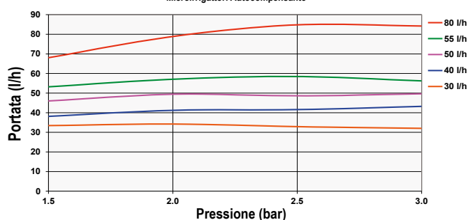
Orbita PC Micro Sprinklers Microirrigatori Autocompensante
